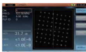
DVB-T2 constellation
