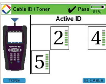
Cable ID mode with Active IDs enables technicians to identify connections for each segment of coaxial cable
