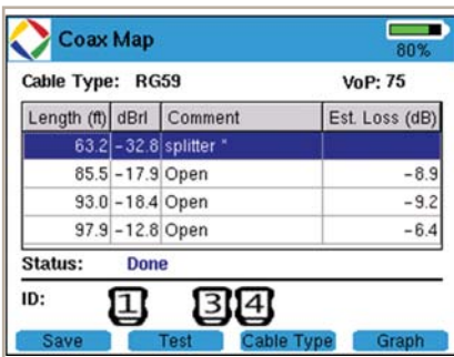
The Coax Map test helps technicians locate and troubleshoot problematic segments of coaxial cable
