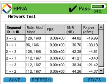
HPNA testing lets users test network metrics between HPNA nodes to verify or troubleshoot HPNA networks
