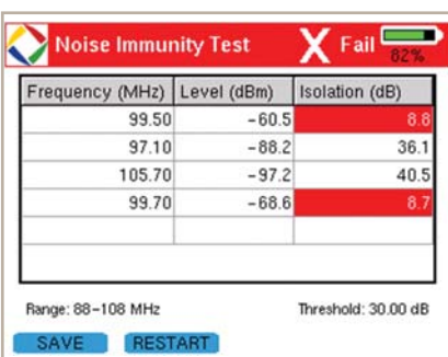
The NIT helps users locate isolation issues in coax cable to identify which legs contain faults that could allow ingress into the coax network
