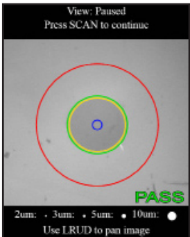
IEC61300-3-35 Auto Pass/Fail Video System
